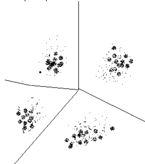
Figure 2: Partitioning Clustering
