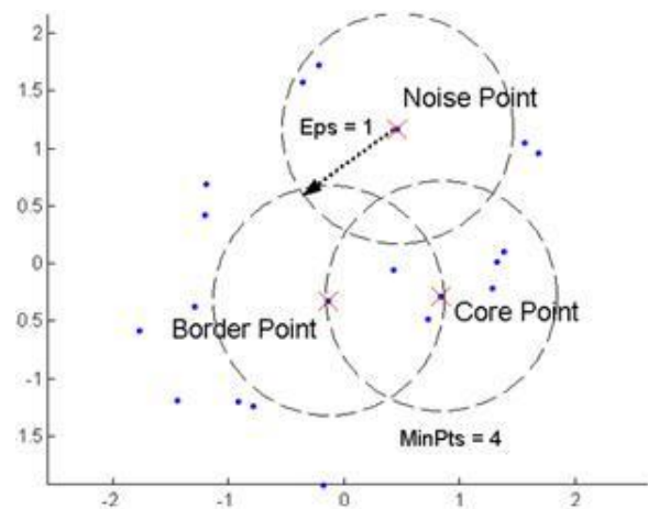
Figure 6: DBSCAN
