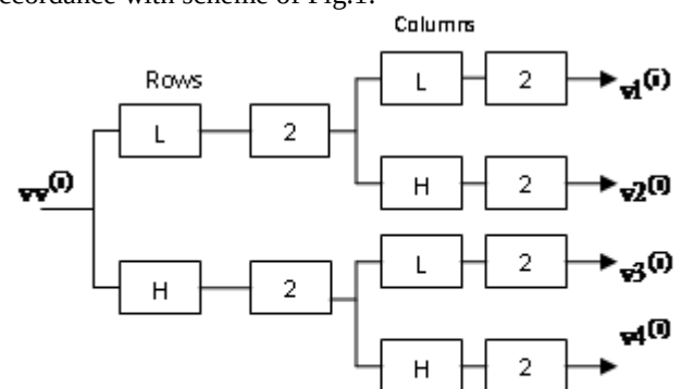
Figure 1: Two-dimensional discrete wavelet transform
