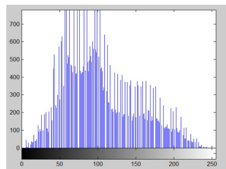
Figure 2: Histogram of the Einstein image
