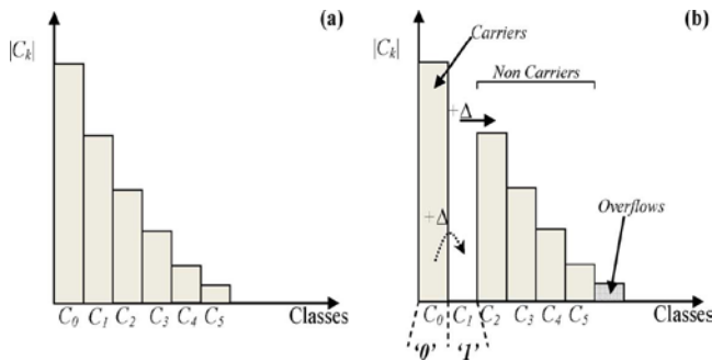
Figure 4: Histogram shifting modulation. (a) Original histogram. (b) Histogram of the watermarked data.
