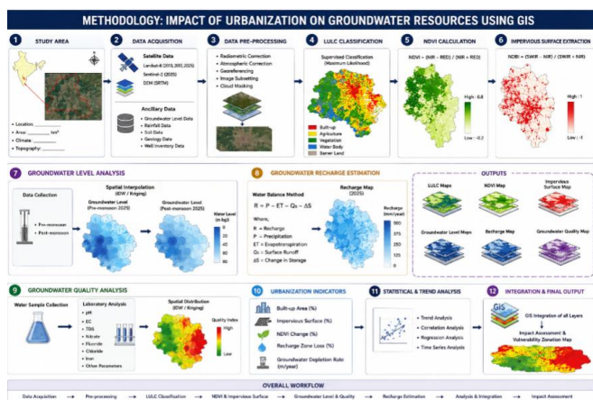
Figure 2: Methodology Framework
