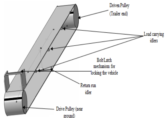
Figure 1: Details of proposed conveyor belt system
