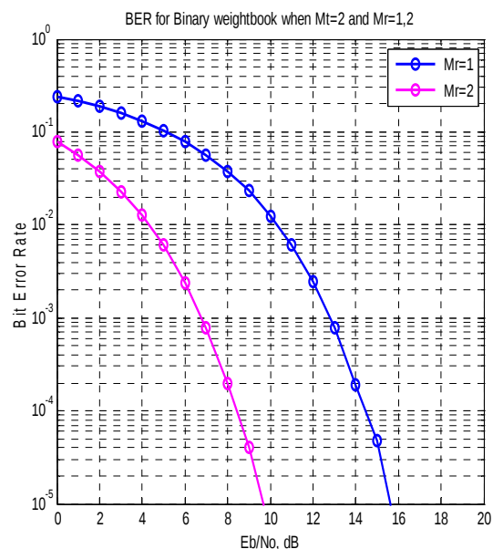
Figure 4.4: Performance comparison of Binary Weightbook when M_r=1, 2 .
