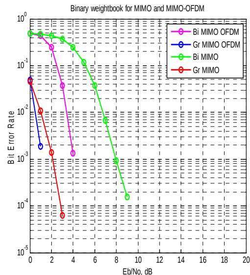
Figure 4.3: Performance Comparison of MIMO and MIMO OFDM.
