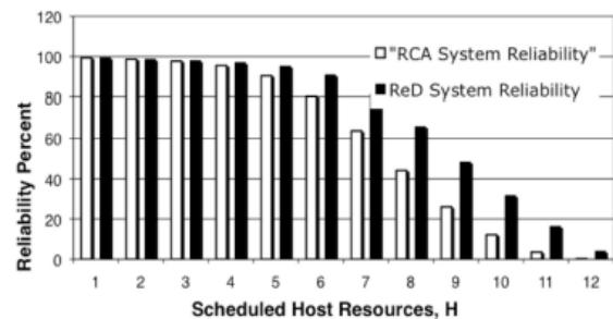
Figure 2: RCA vs. Reliability driven middleware algorithm [1]
