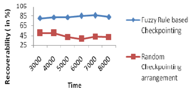
Figure 3: Fuzzy rule VS RCA [7]
