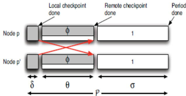
Figure 1: Non blocking Checkpointing Algorithm
