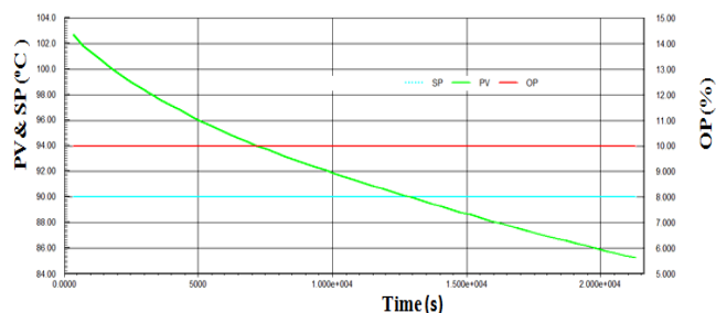
Figure 8: PID control temperature responses to decrease bottom temperature from 104°C to 90°C
