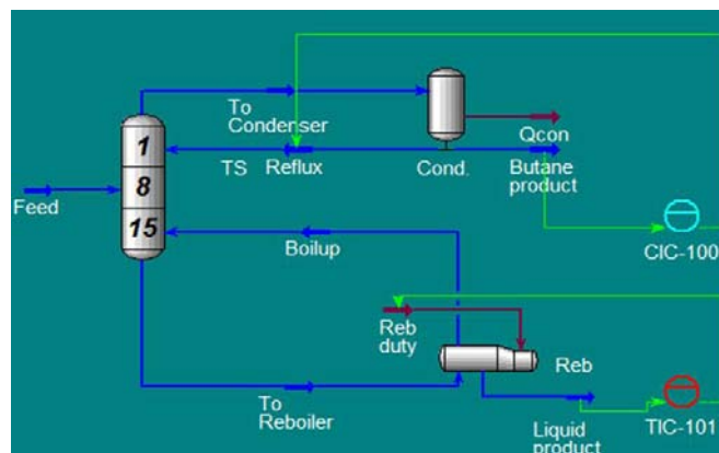
Figure 2: Debutanizer distillation column developed in HYSYS software
