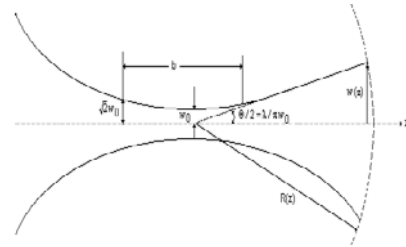
Figure 5: Gaussian beam
