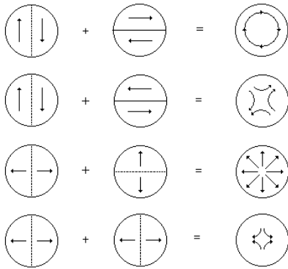
Figure 4: Synthesis of different polarization configurations from the linearly polarized TEM01 mode
