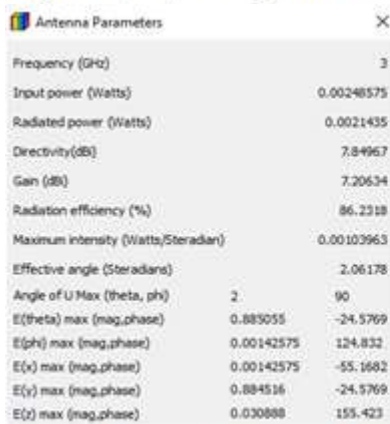
Figure 5: Gain for RT_Duroid5881
