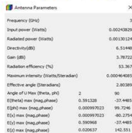
Figure 7: Gain for FR_4
