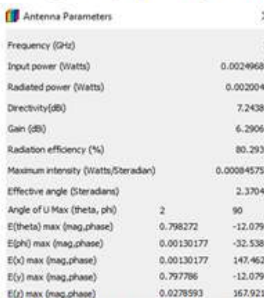
Figure 6: Gain for RT_Duroid6002
