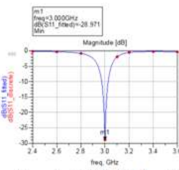
Figure 3: |s11| for RT_Duroid6002
