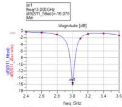
Figure 4: |s11| for FR_4
