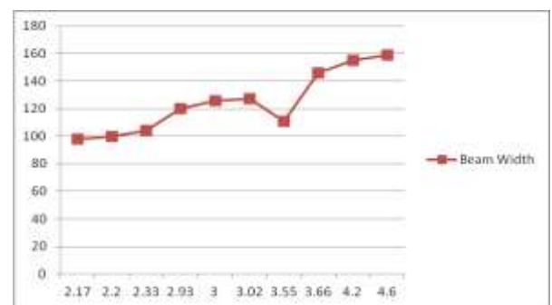
Figure 12: Dielectric constant Vs Beam Width
