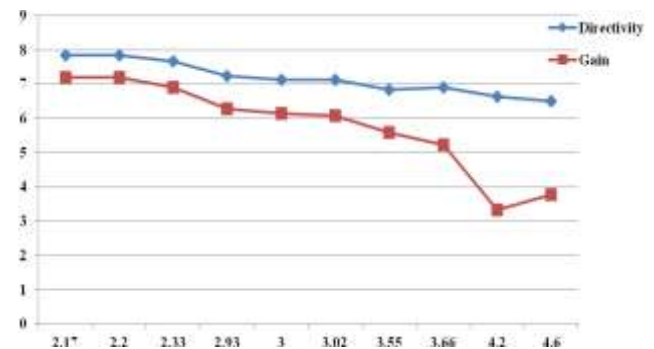
Figure 11: Dielectric constant Vs Gain and Directivity
