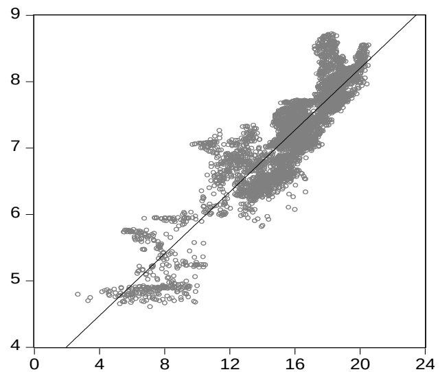
Figure 2: Scatter plot of volume of OLS return and price of Shanghai index
