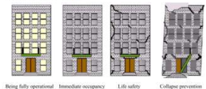
Figure 2: Schematic design of performance levels based on FEMA450
