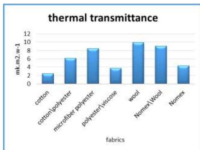
Figure 6: Thermal Transmittance (Rct)
