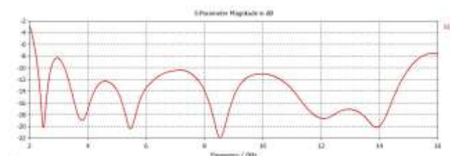
Figure.2. Simulated S11 proposed antenna.
