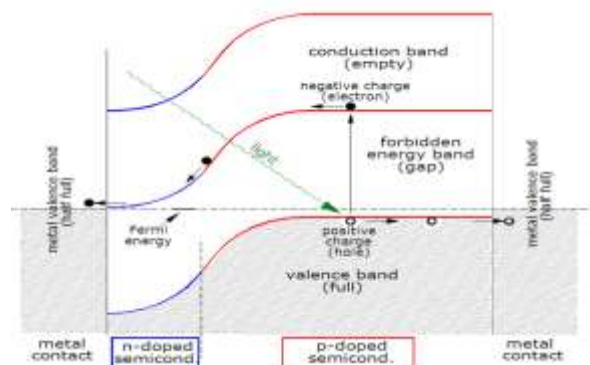
Figure 2: Formation of electron-hole pair.
