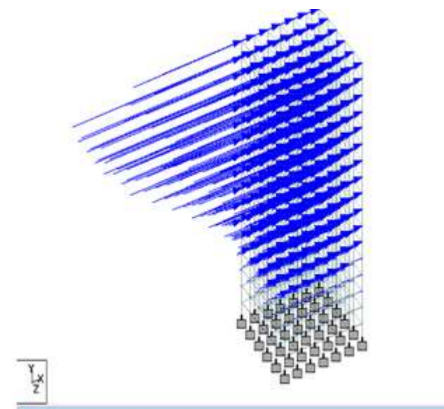
Figure 6: Seismic Loading In Positive X Direction
