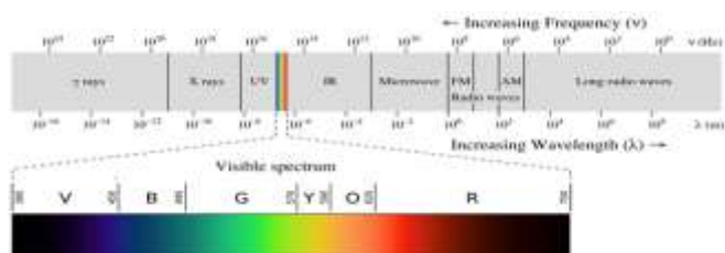
Figure 1: The electromagnetic spectrum
