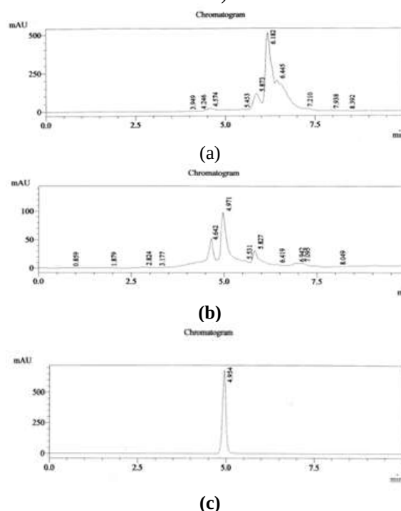
Figure 4: HPLC chromatogram of (a) blank real sample, (b) real sample spiked with 1 \mu\text{g.mL}^{-1} (c) pyroxsulam standard solution
