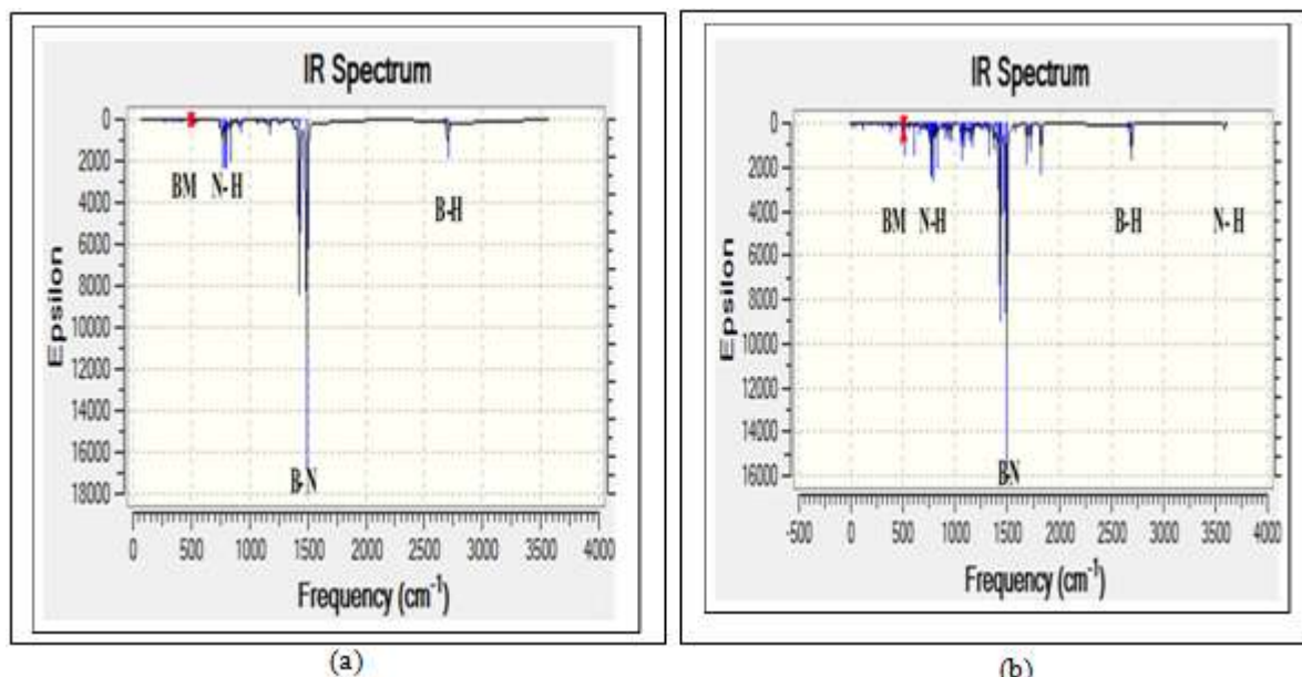
Figure 2: Calculated IR spectra of molecules, (a) SWBNNT, (b) SWBNNT with 5-Fu.Using B3LYP/6-31G (d) method.
