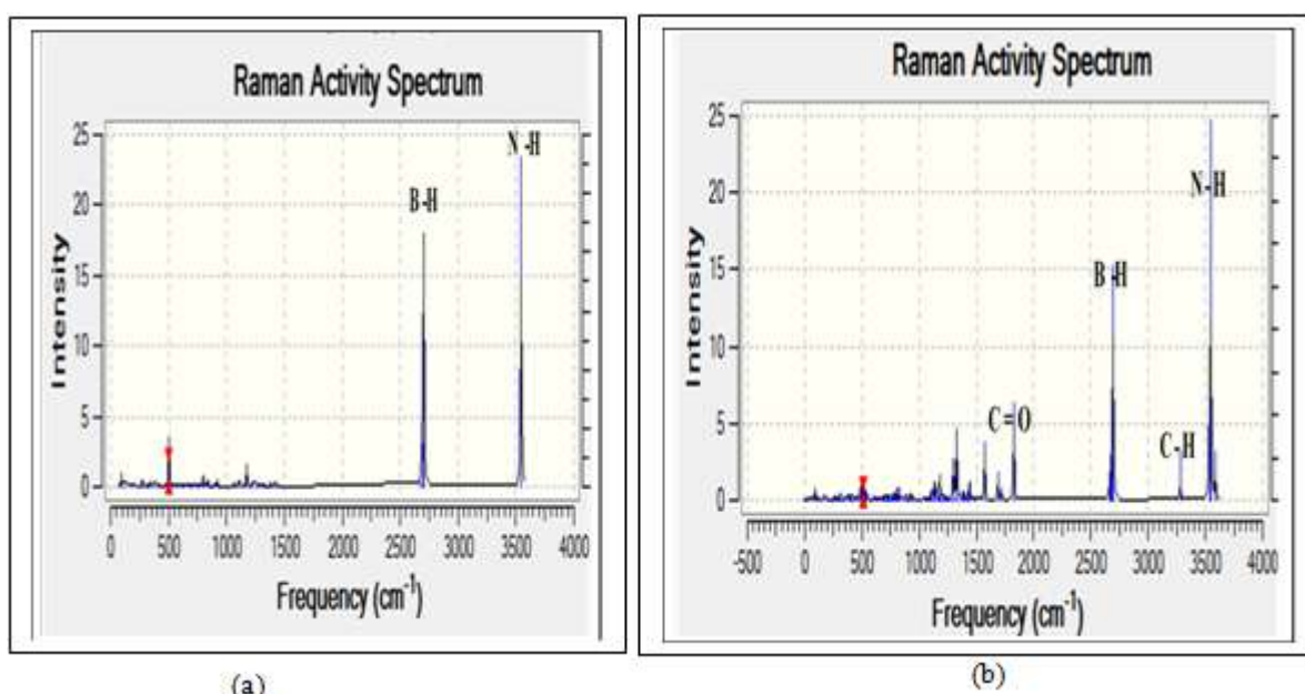
Figure 3: Calculated Raman spectra of molecules, (a) SWBNNT, (b) SWBNNT with 5-Fu.using B3LYP/6-31G (d) method
