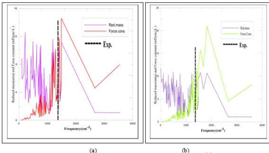
Figure 4: Reduced Masses and Force Constant as a function of frequency for: (a) SWBNNT and (b) Complex. The dashed line represents the bulk BN LO vibration frequency [21].
