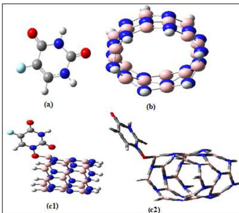
Figure 1: The structures of optimized molecular by B3LYP/6-31G (d) method. (a) 5- FU, (b) Nanotube (6, 0), and the complex (c1 as ball and bond, c2 as tubes).
