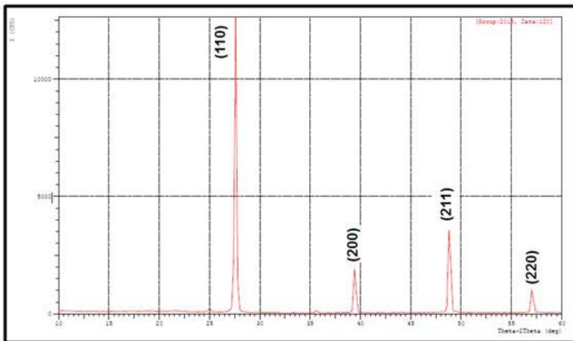
Figure 2 (d): X-ray diffraction pattern of CsI film deposited at (200°C) doped with (0.75)ml KI
