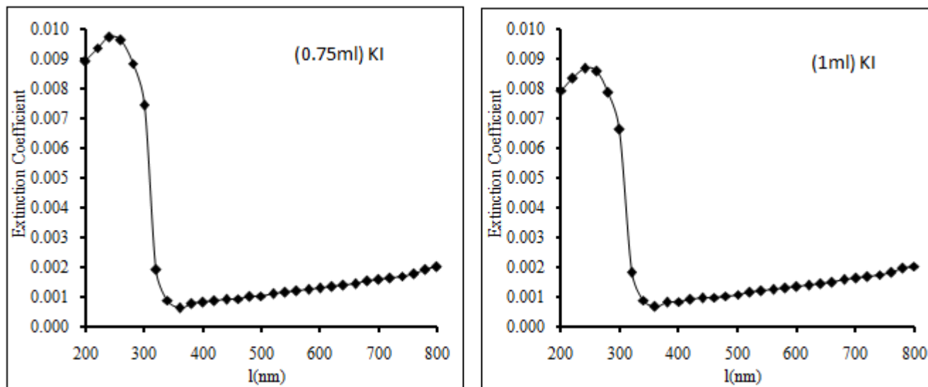
Figure 8: Extinction coefficient plots of CsI films with different doping concentrations
