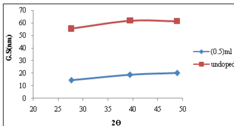
Figure 11: Grain size curves for CsI angular dependence of undoped and doped samples
