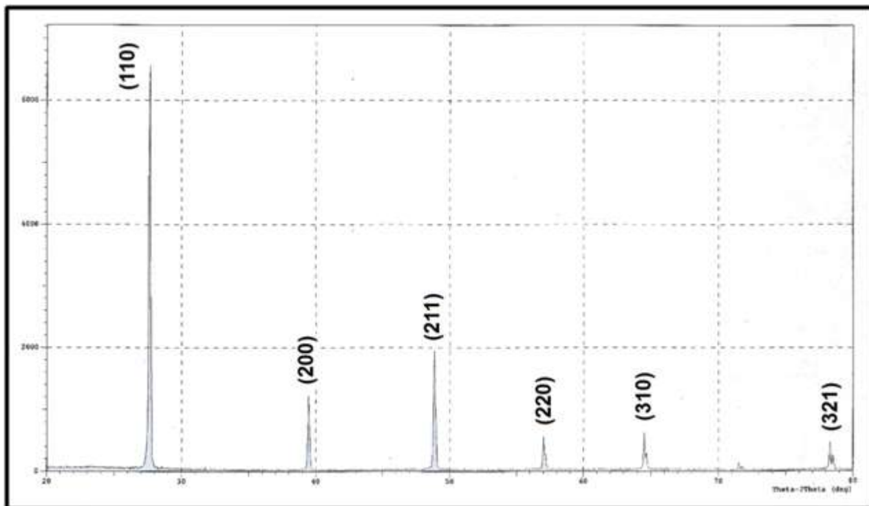
Figure 2 (a): X-ray diffraction pattern of undoped CsI film deposited at (200°C)
