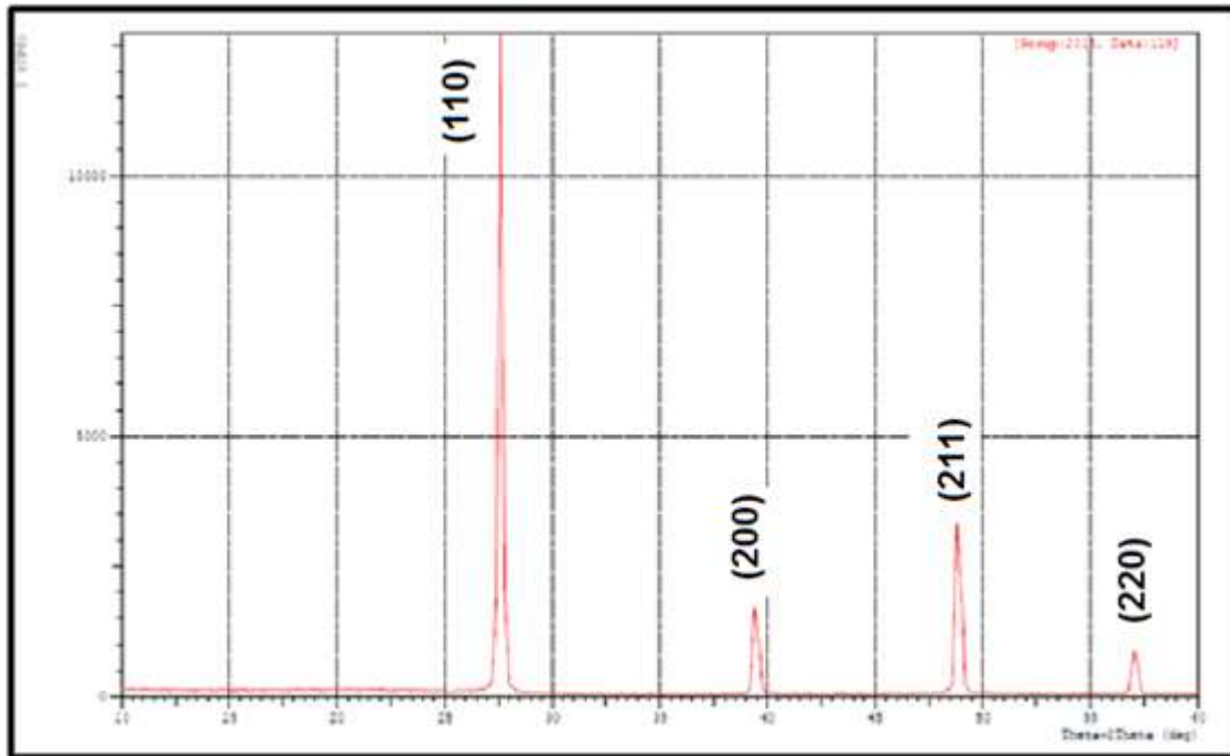
Figure 2 (c): X-ray diffraction pattern of CsI film deposited at (200°C) doped with (0.5)ml KI
