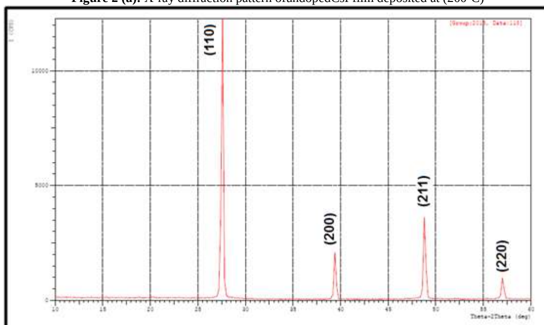
Figure 2 (b): X-ray diffraction pattern of CsI film deposited at (200°C) doped with (0.25)ml KI
