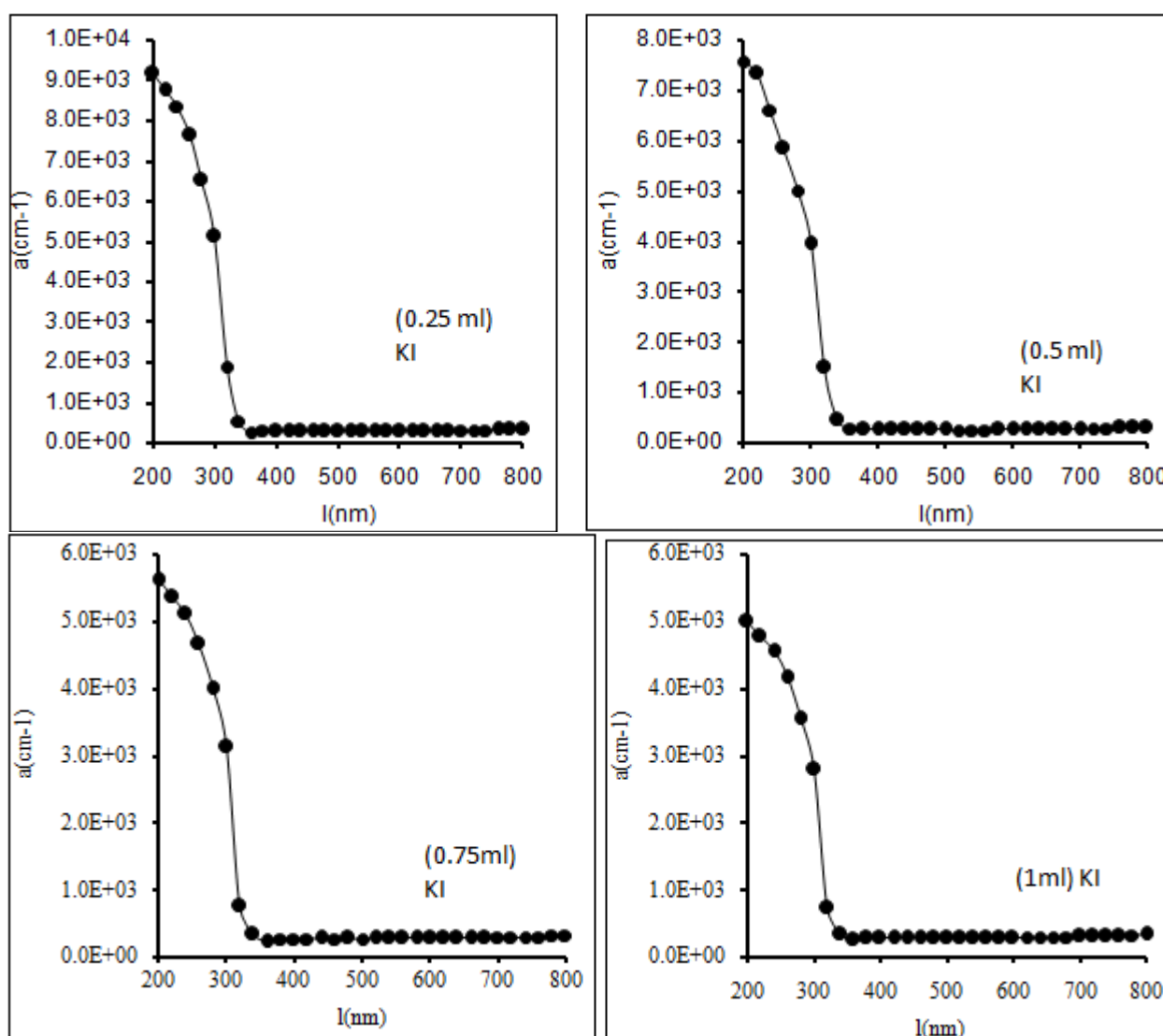
Figure 9: Absorption Coefficient plots of CsI films with different doping concentrations
