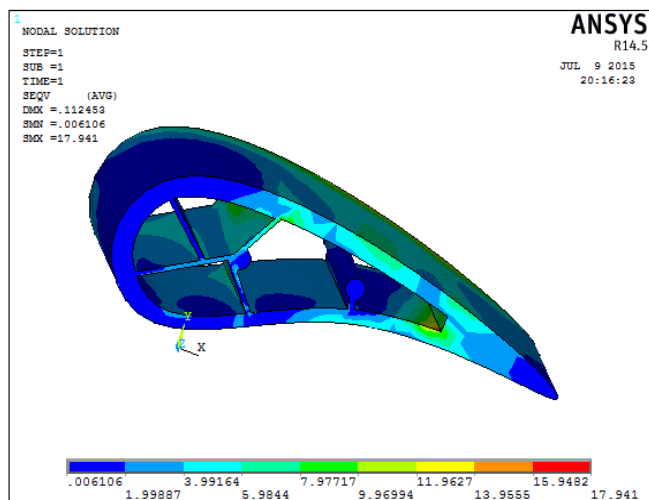
Figure 6: Stress analysis for NIMONIC 901 blade
