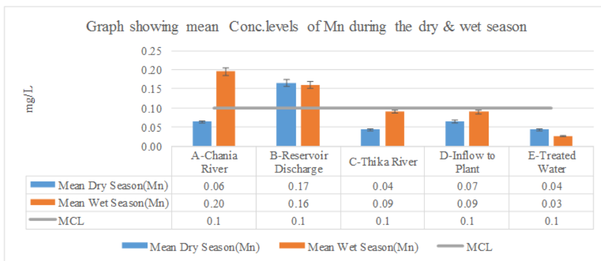
Figure 4: Concentration of manganese during wet and dry seasons
