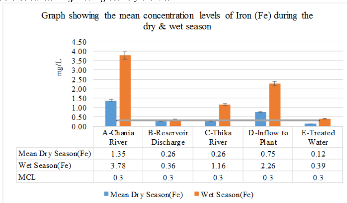
Figure 3: Iron concentration during dry and wet seasons
