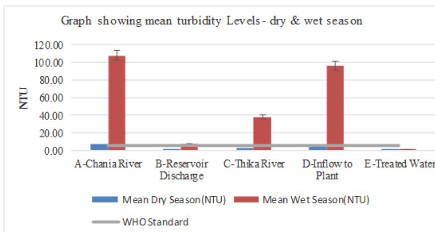
Figure 2: Turbidity levels during the wet and dry seasons
