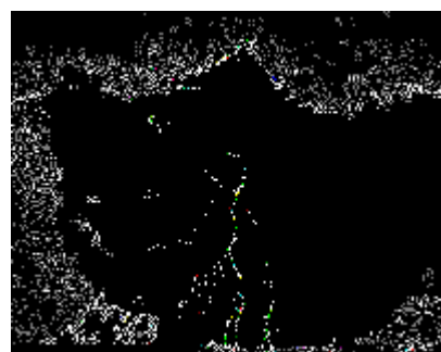
Figure 6: Wavelet image
