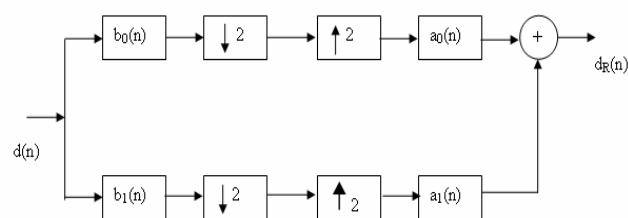
Figure 5: Two channel wavelet structure
