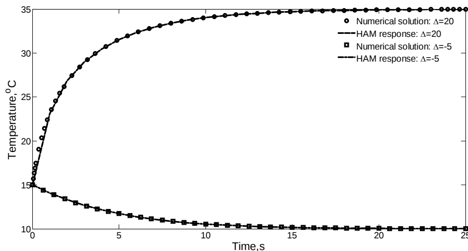
Figure 4: Comparison between the HAM predicted dynamics vs. the actual response for the step changes of different amplitude and direction
