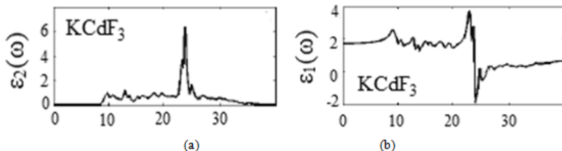
Figure 3: The calculated (a) imaginary \varepsilon_2(\omega) and (b) real \varepsilon_1(\omega) parts of complex dielectric constant of KCdF 3 perovskites.
