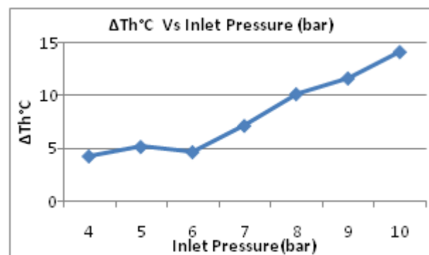
Figure 8 Increase in \Delta T_h with increase in inlet pressure
