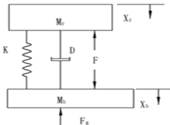
Figure 3: The dynamical model of vibrator
