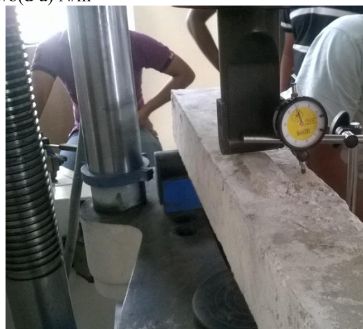
Figure 3: Fracture energy test
