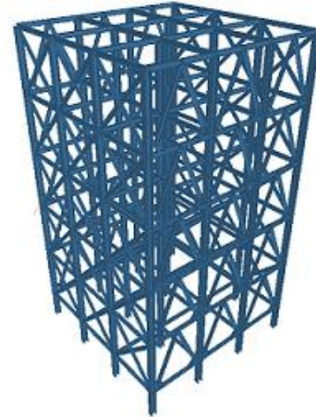
Figure 8: X and Knee type bracing
