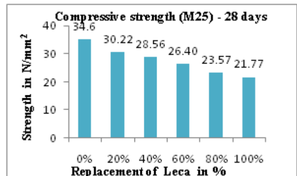
Figure 4: Compressive strength comparison of L1 & L3
