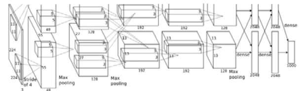
Figure 3: Depicting the structure of network used by Hinton, Krizhevsky and Sutskever in their classification experiment. [2]
