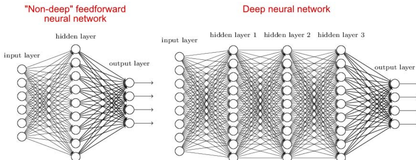
Figure 1: shows the difference between neural network and Deep Neural Network. [1]
