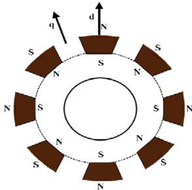
Figure 1: Surface PM (SPM) Synchronous Machine
