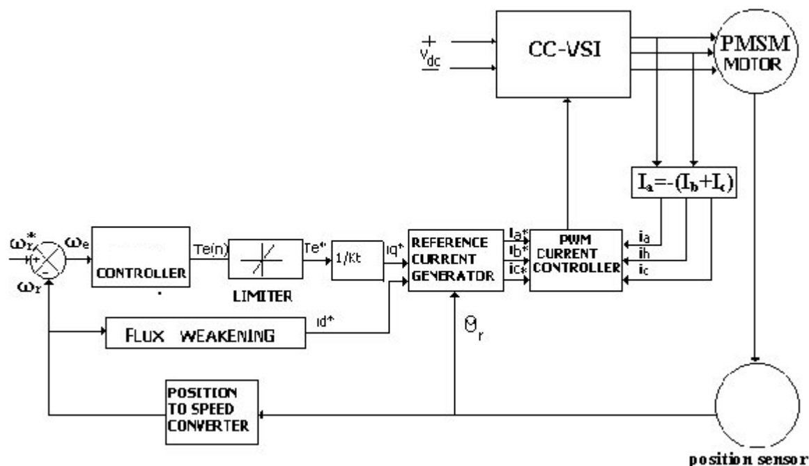
Figure 3: Schematic Block Diagram of PMSM Drive
