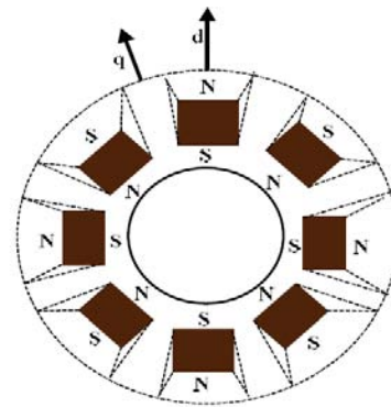
Figure 2: Interior PM (IPM) Synchronous Machine
