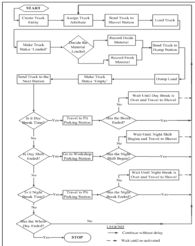
Figure 1: Conceptual model of shovel-truck system
