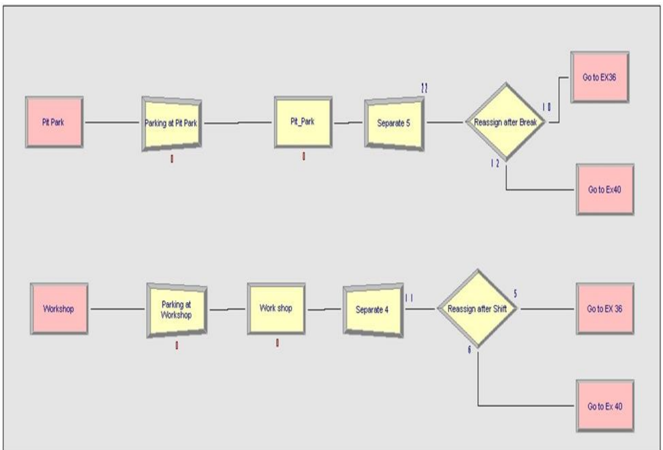
Figure 2.3: Break times modelling
