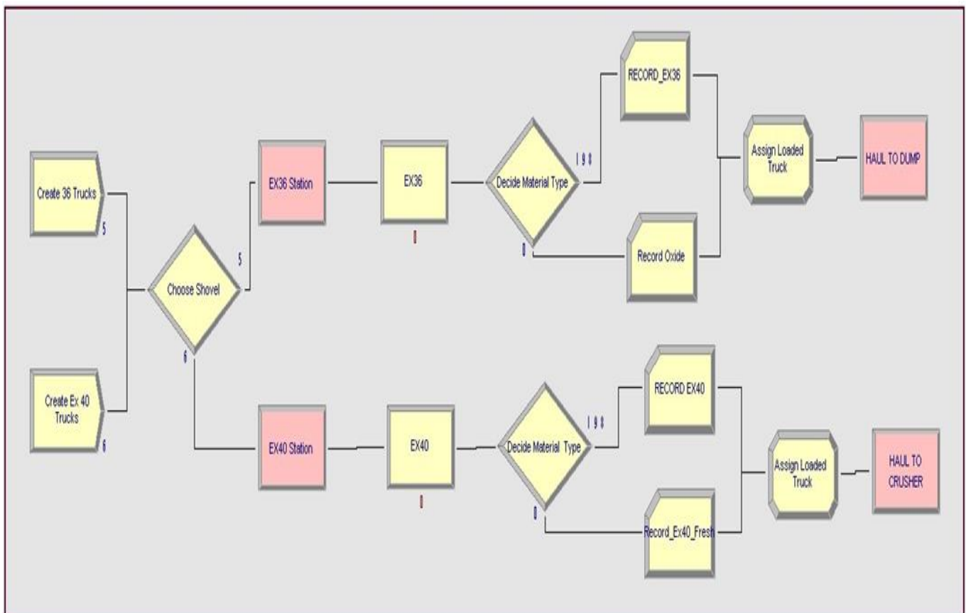
Figure 2.1: Trucks Entities creation and shovel Processes
