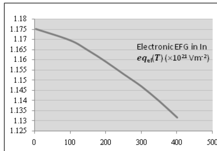
Figure 2: Electronic EFG in Indium as a function of temperature in Kelvin
