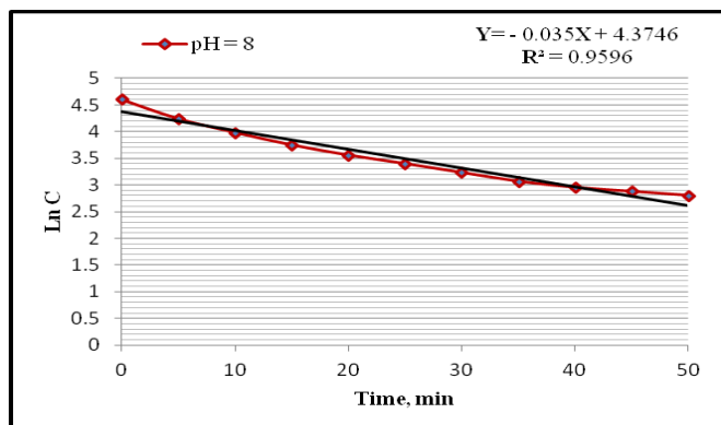
Figure 4.6: First order reaction curve for the adsorption kinetics of sodium dodecyl Sulfate on copper surface for initial concentration is 75 mg/L and pH = 8.
