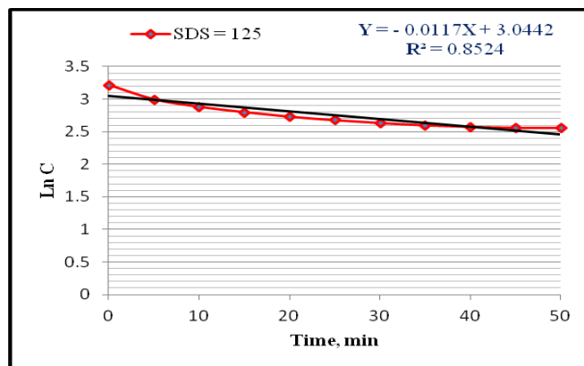
Figure 4.3: First order reaction curve for the adsorption kinetics of sodium dodecyl Sulfate on copper surface for initial concentration is 125 mg/L.
