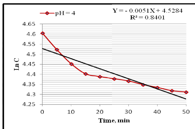
Figure 4.4: First order reaction curve for the adsorption kinetics of sodium dodecyl Sulfate on copper surface for initial concentration is 75 mg/L and pH = 4
