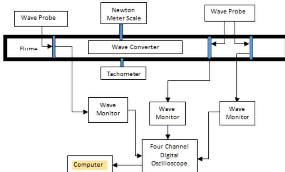
Figure 2.1: Block diagram of the experiment
