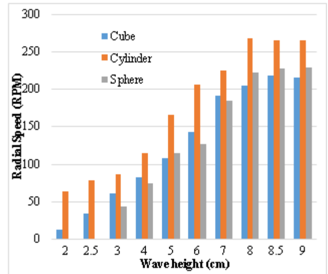
Figure 3.2: Wave height and radial speed of flywheel shaft on different container shape
