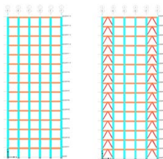
Figure 2: Showing the elevation in XZ view of Model 1 & Model 2
