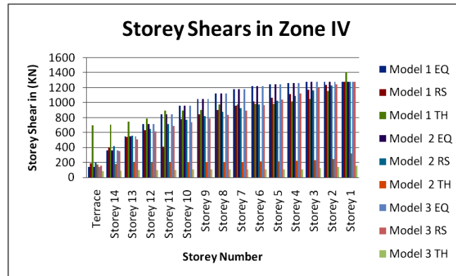
Chart 4: Showing Storey Shears in Zone IV
