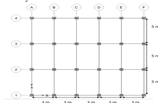
Figure 1: Showing the plan of a G+14 building
