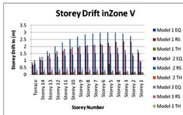
Chart 3: Showing Storey Drift in Zone V
