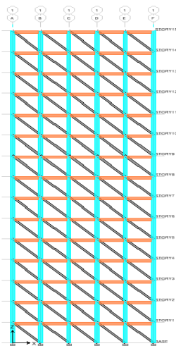
Figure 3: Showing the elevation in XZ view of a Model 3
