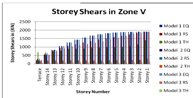
Chart 5: Showing Storey Shears in Zone V
