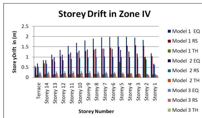
Chart 2: Showing Storey Drift in Zone IV
