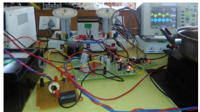
Figure 11: Experimental Set-up of Full Bridge AC-AC Resonant Converter.
