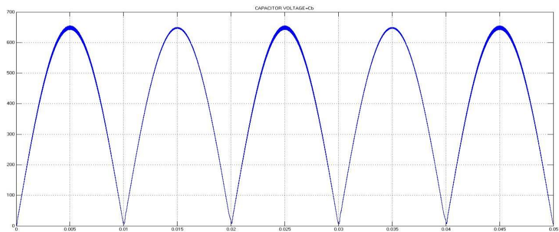
Figure 9: Simulated Waveform of Capacitor Voltage
