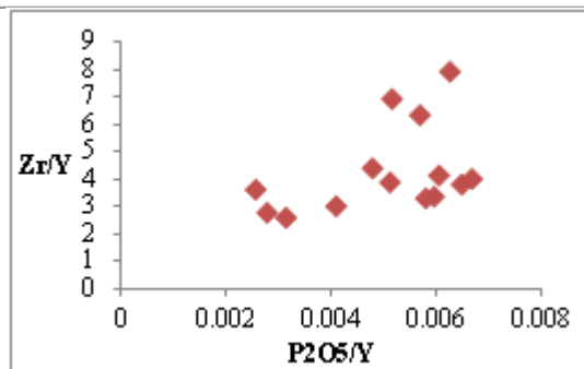
Figure 19: P_2O_5/Y Vs. TiO_2/Y and Zr/Y variation
