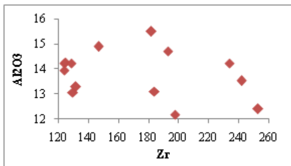
Figure 9: Zr vs. Al_2O_3
