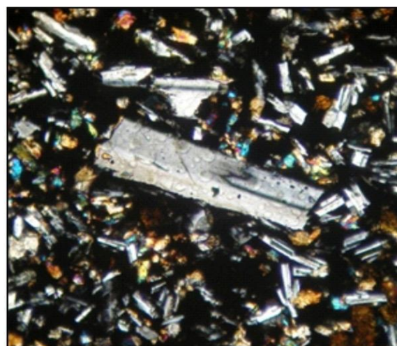
Figure 4: Corroded border in Plagioclase
