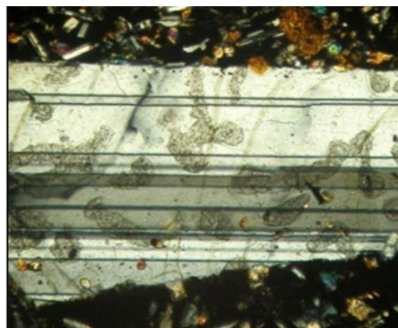
Figure 3: Plagioclase occurring as Phenocryst
