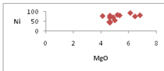
Figure 12: MgO vs. Cr, Ni
