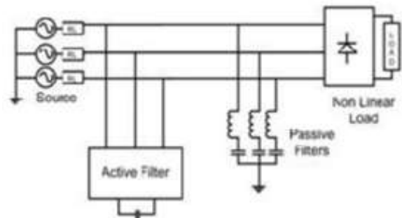
Figure 4: Hybrid Filter in power system.
