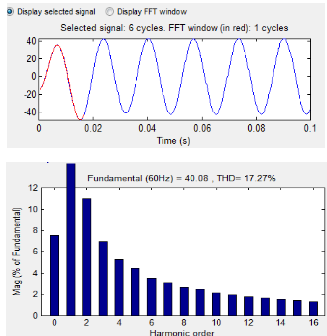
Figure 9: Harmonic analysis for the output current with filter
