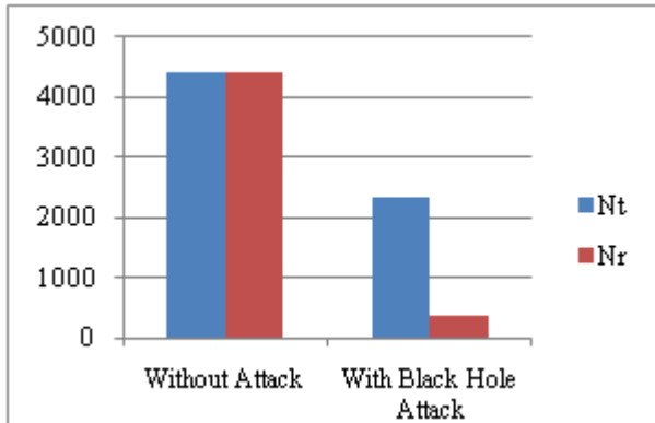
Figure 5.2: Comparison between delivery ratio of network with and without black hole attack
