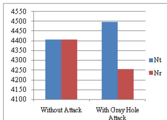
Figure 5.1: Comparison between delivery ratio of network with and without gray hole attack
