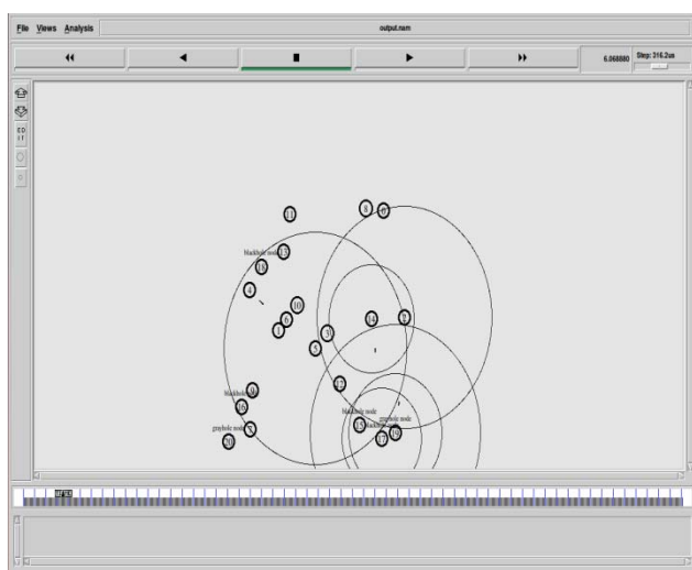
Figure 4.2: Simulation in NS2 with presence of Gray hole attack
