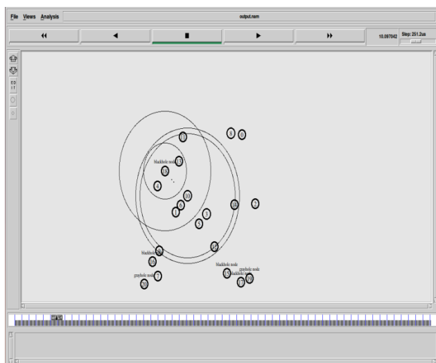
Figure 4.3: Simulation in NS2 with presence of Black hole attack
