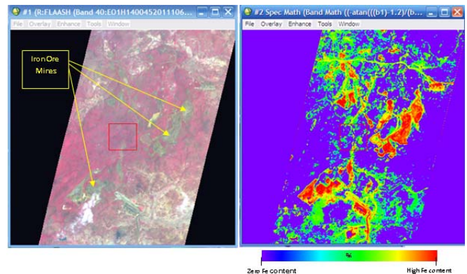
Figure 4: Showing the final result of Fe distribution of Noamundi areas. Hyperion Image (Left) and Fe distribution areas (Right)
