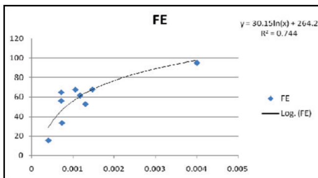
Figure 3: Field Fe content versus spectral iron parameter ( \theta Fe)
