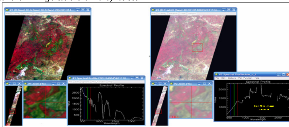
Figure 2: Showing the spectral profile of Iron ore mining areas of before and after atmospheric Correction. Hyperion Image before (Left) and after (Right) atmospheric Correction
