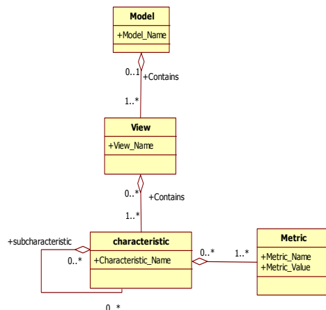
Figure 2: Our Meta-model for software quality
