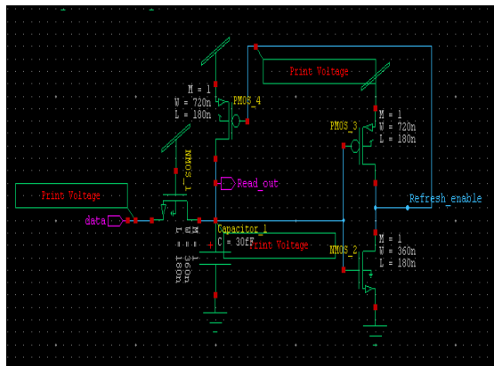
Figure 3: DRAM cell with only refresh circuitry
