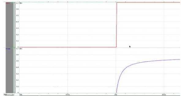
Figure 19: Write cycle of 1T1C DRAM
