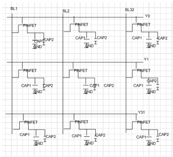
Figure 8: 1KB DRAM memory
