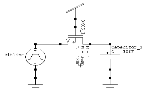
Figure 1: Schematic of 1T1C DRAM cell
