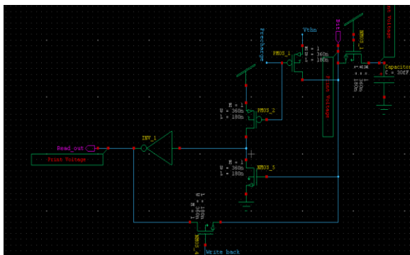
Figure 4: Read scheme of 1T1C DRAM using two cascaded inverters
