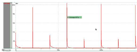
Figure 23: Average power consumption of read cycle of 1KB DRAM memory
