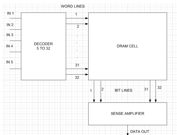
Figure 9: 1KB DRAM memory
