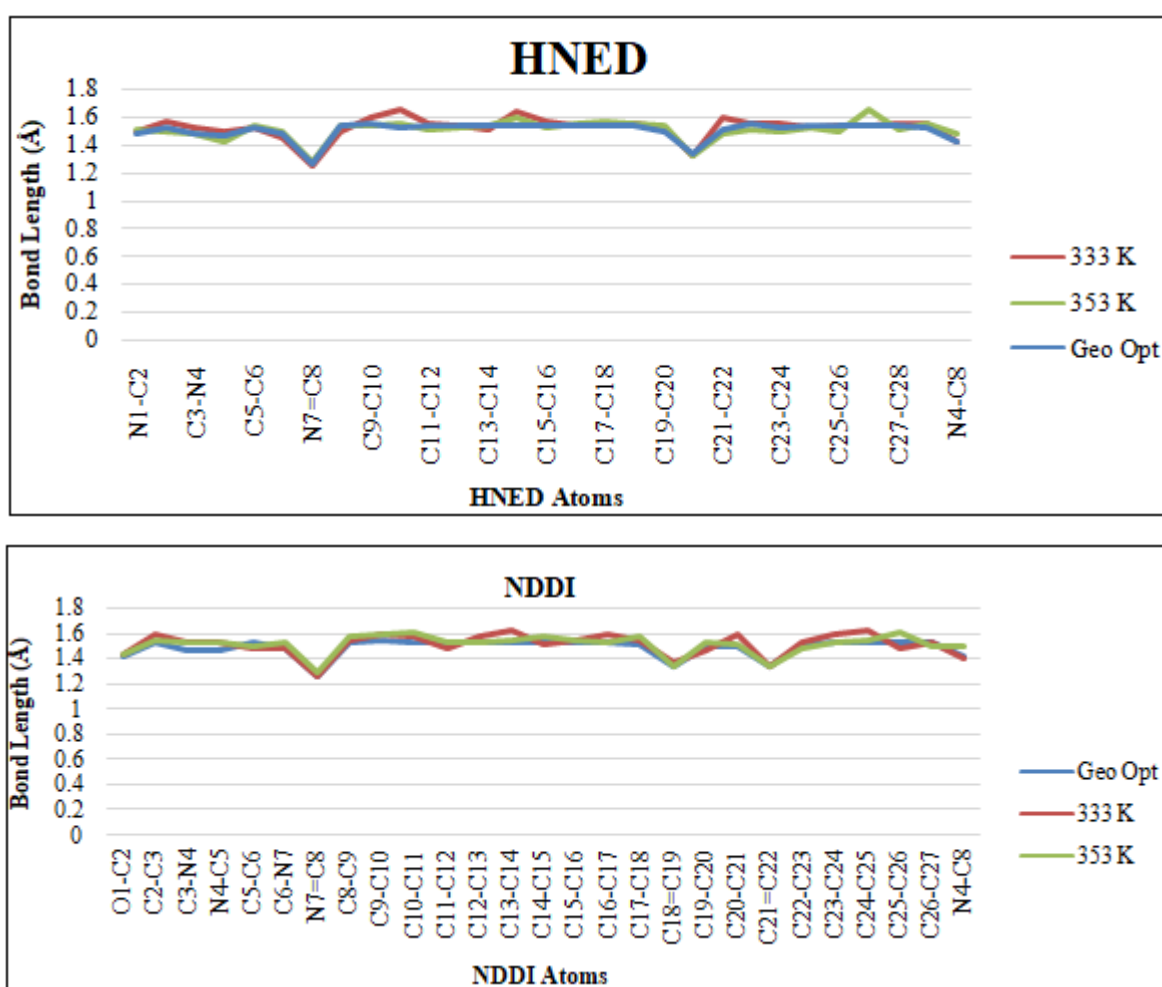
Figure 3: Bond length analysis for HNED and NDDI at Geometry Optimization, 333 K and 353 K
