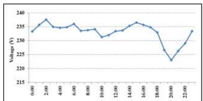
Figure 6: Voltage profile without solar PV
