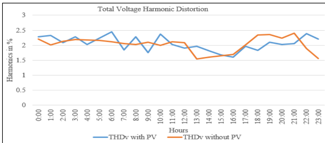
Figure 13: Voltage THD
