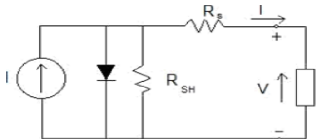
Figure 1 : Electrical Equivalent Circuit Model of PV Cell
