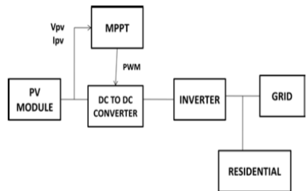
Figure 3 : Block diagram of grid connected PV system
