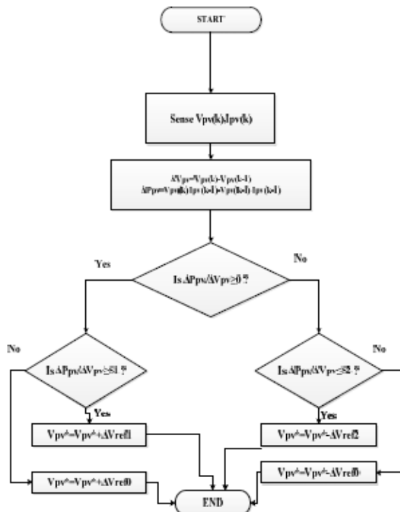
Figure 2 : Flowchart of P&O algorithm
