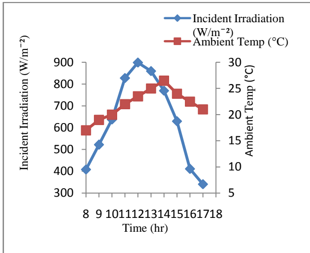
Figure 3: Instantaneous irradiation and ambient temperature for Solar water flat plate collector
