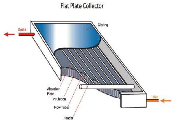
Figure 2: Cross sectional area of flat plate collector
