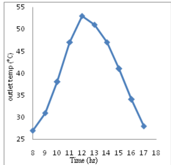
Figure 5: variation of outlet temp with time for 0.01 kg/s mass flow rate with insulation
