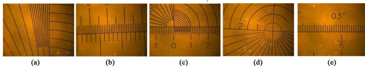
Figure 2. Optical micrographs of some of the metric and multi-gauge touch reticles used for patterning and immobilization of RhB molecules on polybutadiene covered glass slide.
