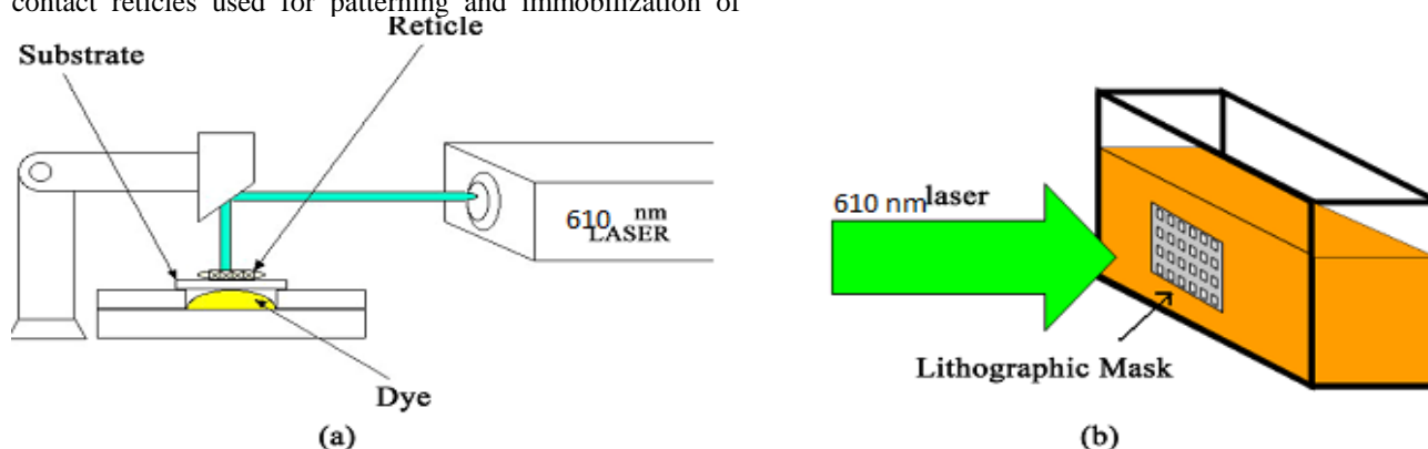
Figure 1: Schematic experimental set-up for laser micro-printing and immobilization of RhB dye and other biomolecules on polymer substrates (a). The change set-up the usage of aqueous cell (b) packed with dye-answer.
