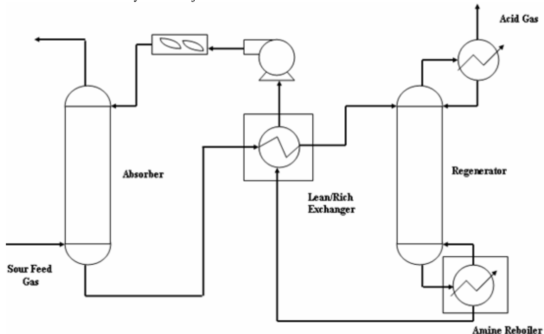
Figure 3. Schematic of a simple amine unit.
