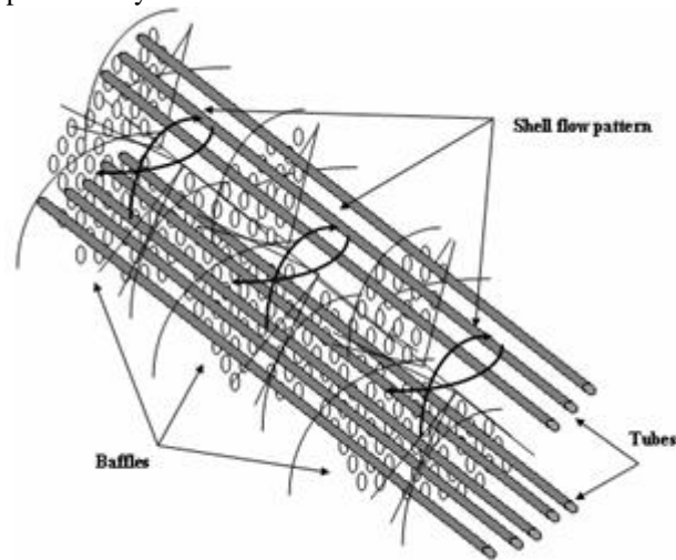
Figure 2. Schematic of helical baffles.
