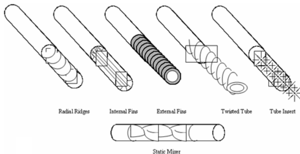
Figure 1. Examples of tubes with heat transfer enhancement.
