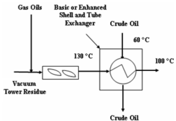
Figure 4. Schematic of a Crude Preheat unit.
